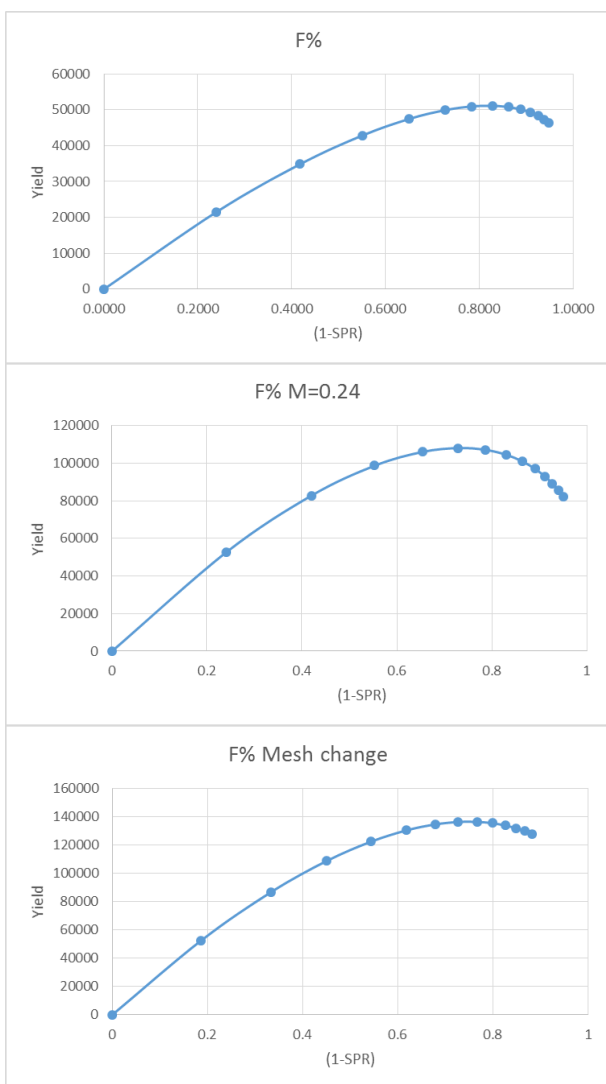
Figure 2.1.3. North Sea cod. The sensitivity of (1-SPR) msy to M at age used and mesh size changes. Top panel based on ICES (2017) data, middle panel, M=0.24 for all ages, and bottom panel M=0.24 and exploitation pattern shifted one age group “down” simulating a mesh size increase.
